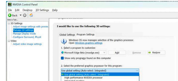
Figure B - 25 Program Settings (Windows Graphic Settings)
